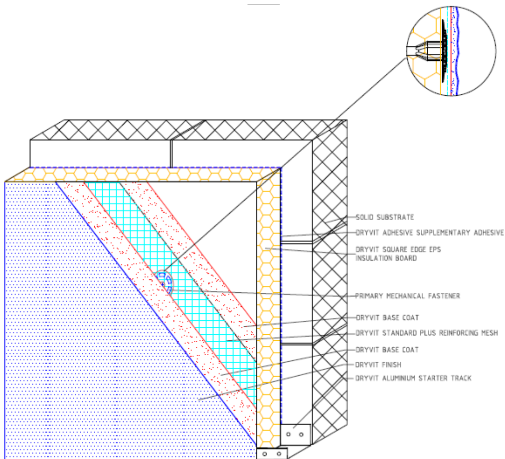
Figure 3b: Outsulation® Plus primary mechanical fix and supplementary adhesive with fixings below the mesh
